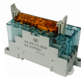
patice A6-6Z-C2
