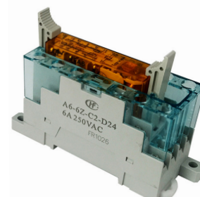
patice A6-6Z-C2
