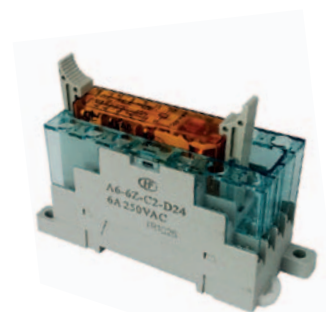
patice A6-6Z-C2
