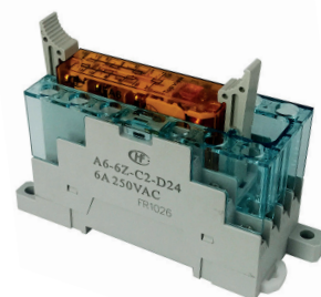
patice A6-6Z-C2
